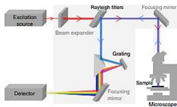
Figure 2. Internal components of the Raman device [1].
