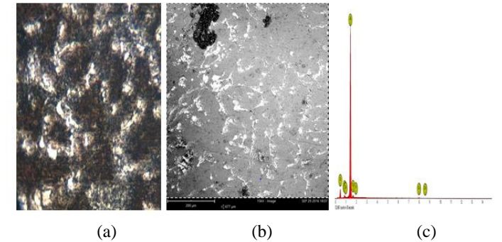
Figure 8. (a) Optical Micrograph (b) SEM Micrograph (c) EDS spectrum of Al 6wt. % Cu at 96 mm/s
