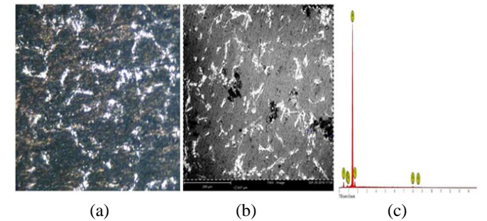
Figure 6. (a) Optical Micrograph (b) SEM Micrograph (c) EDS spectrum of Al 6wt. % Cu at 60 mm/s
