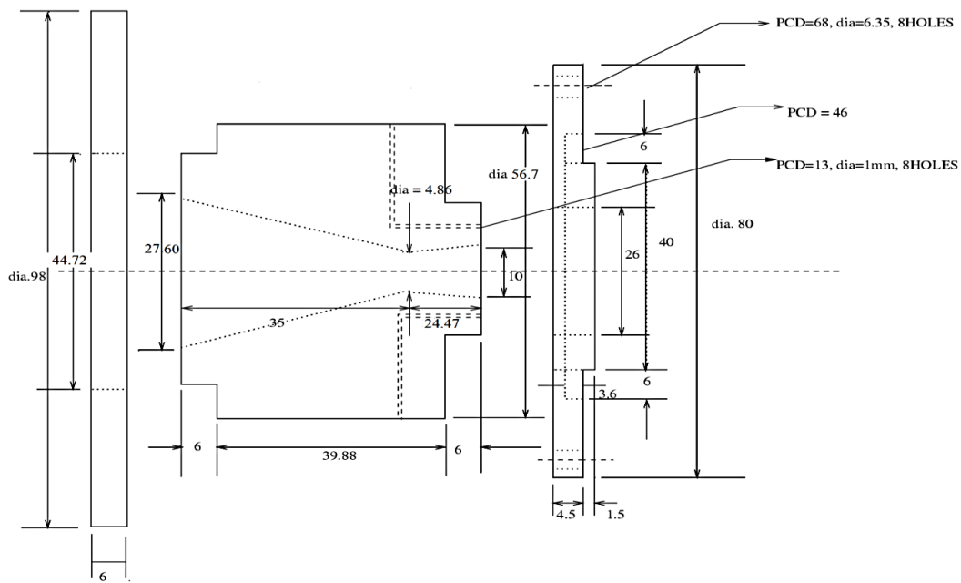
Figure 2. Nozzle design for Mach 3.0.
