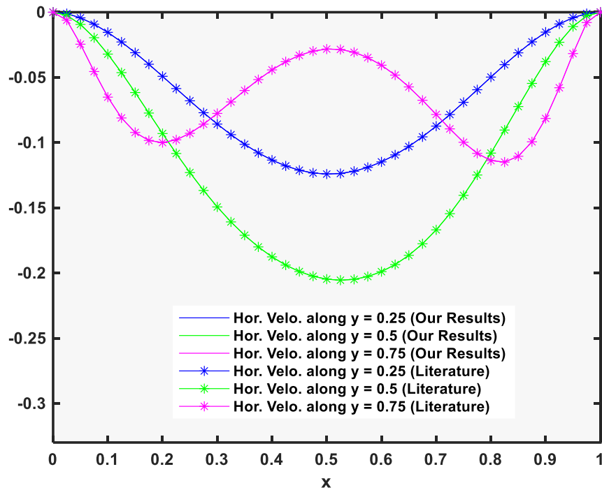
Fig. 3. Validation of the Present Numerical Results Through Comparison with the Analytical Solution Reported by Shih and Tan [40].
