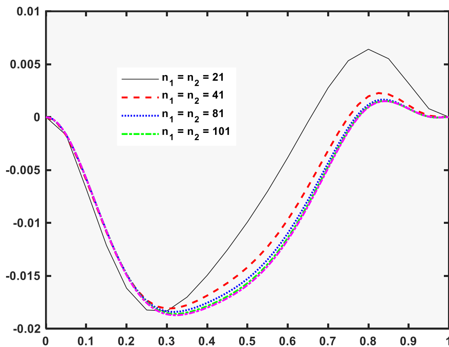
Fig. 4 Study of Mesh Sensitivity for a Normal Velocity Distribution
