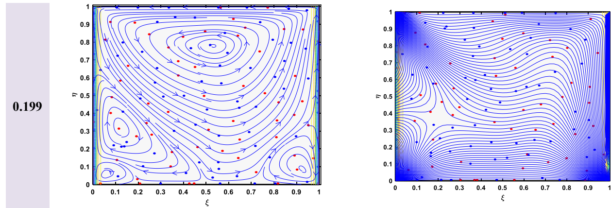
Fig. 7. Visualization of Flow Patterns through Streamlines and Isotherms at Various Widths of Magnetic Field (L).
