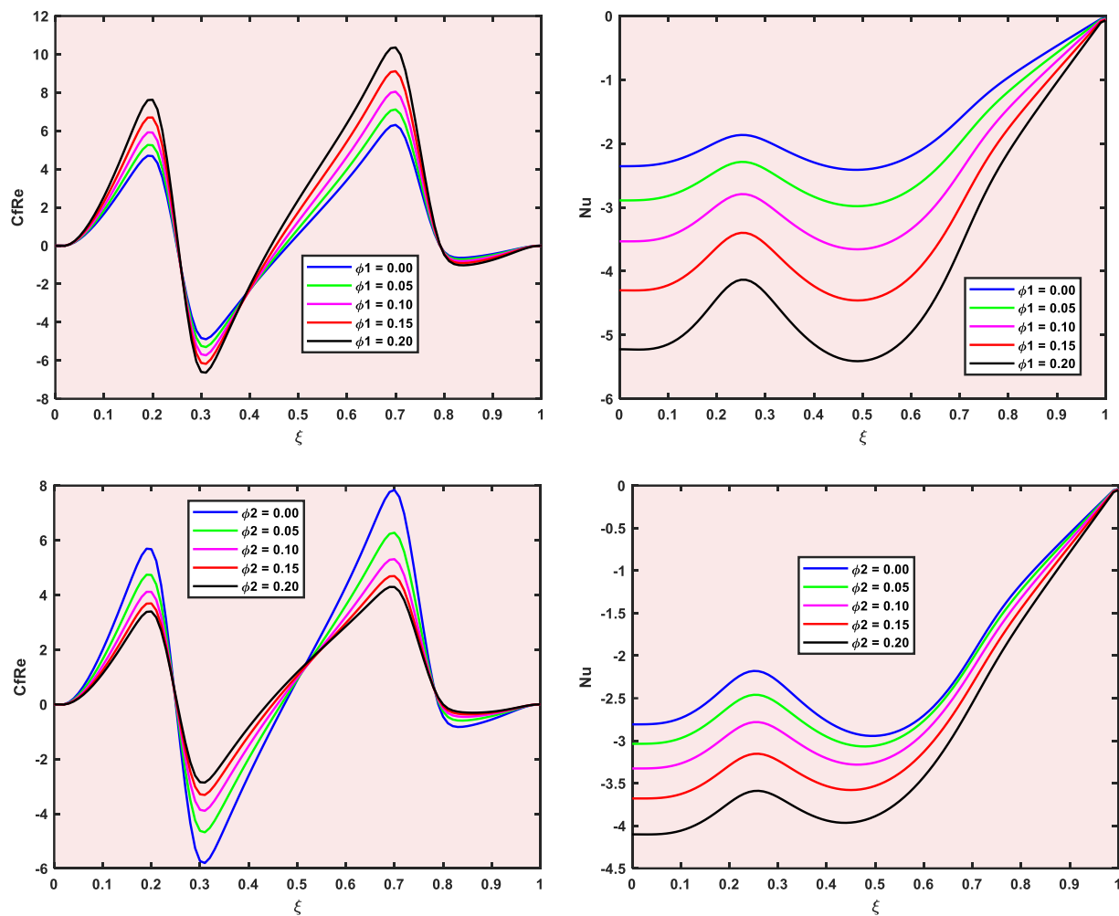
Fig. 8. Variations in Skin Friction (CfRe) and Nusselt Number (Nu) Across Different Parameters
