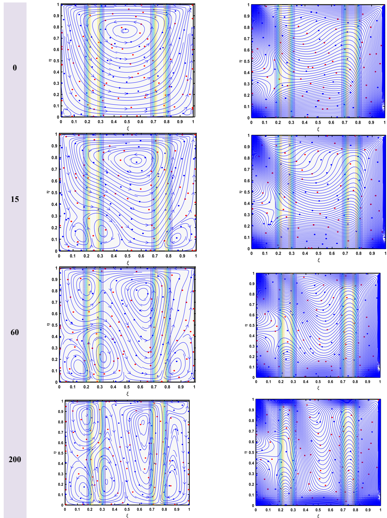
Fig. 5. Visualization of Flow Patterns through Streamlines and Isotherms at Various Mn .
