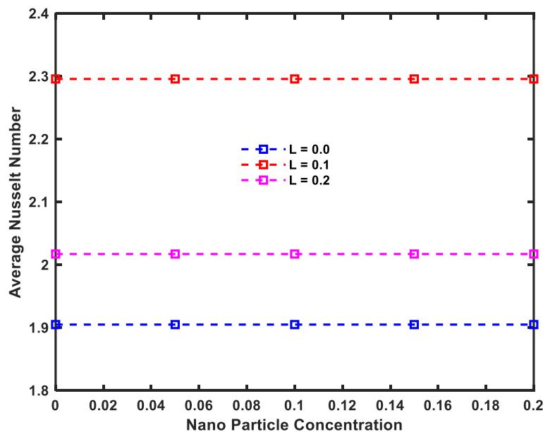
Fig. 11. Influence of Localized Magnetic Strip Width on the Average Nusselt Number
