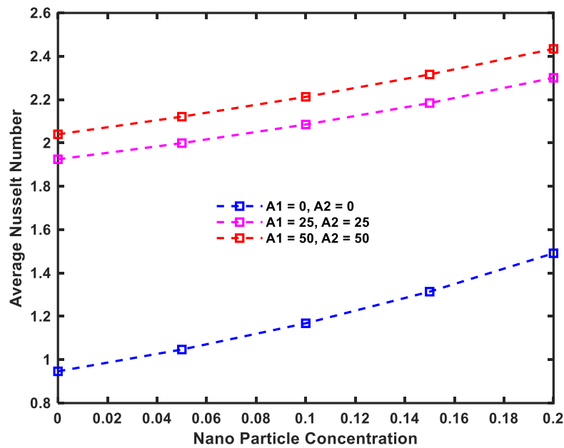
Fig. 10. Effect of Magnetic Field Intensity Parameters A_1 and A_2 on the Average Nusselt Number
