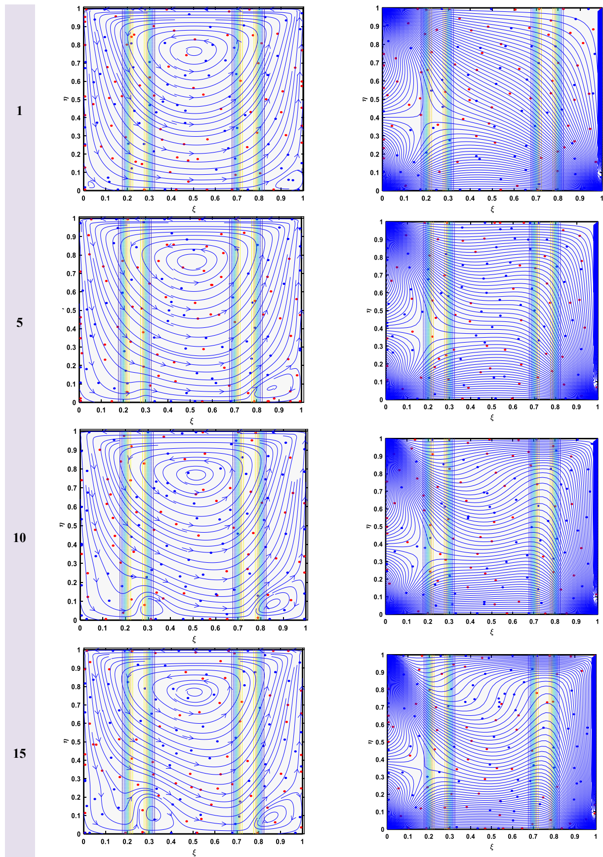
Fig. 6. Visualization of Flow Patterns through Streamlines and Isotherms at Various Re.
