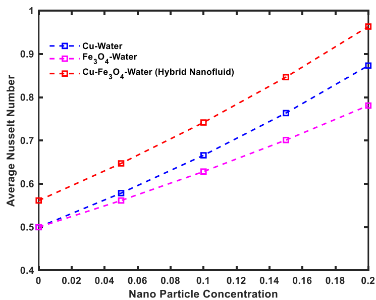
Fig. 9. Comparative Assessment of Thermal Performance Between Individual Nanoparticles and Hybrid Nanofluids
