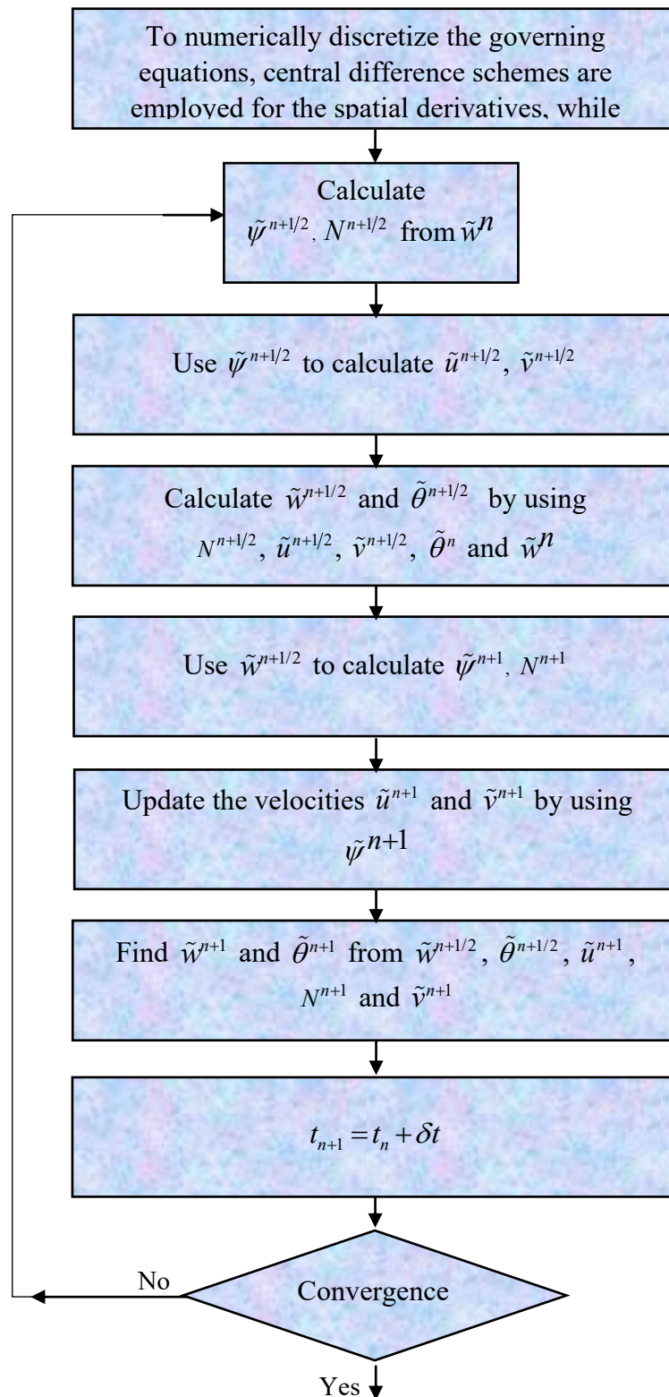
Fig. 2. Flow Diagram of the Pseudo-Transient Numerical Procedure
