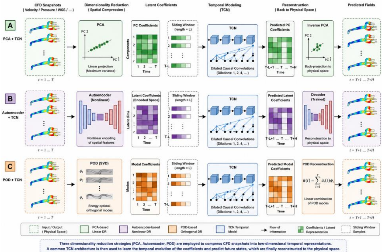
Fig. 5: Schematic representation of the three reduced-order modeling and temporal-prediction frameworks employed in this study: (A) PCA–TCN, (B) Autoencoder–TCN, and (C) POD–TCN.
