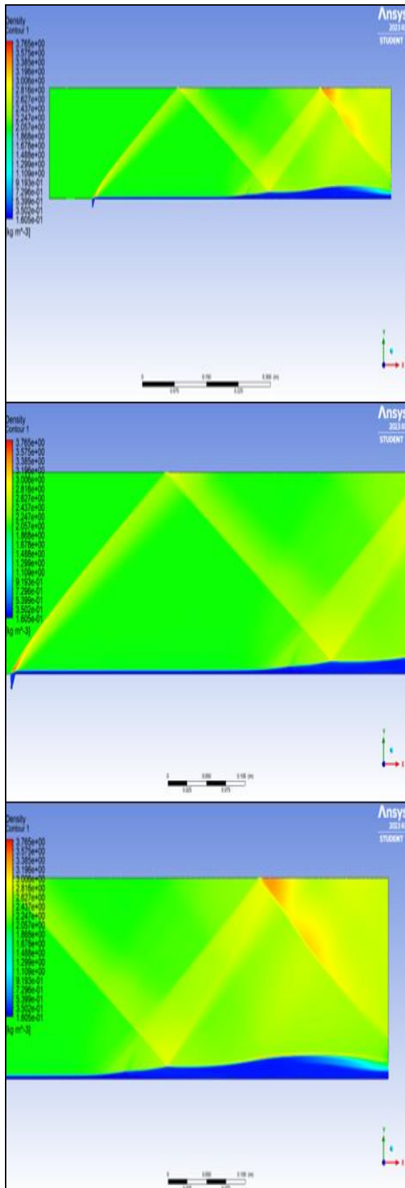
Fig 12: Density contours (Case 2) (top full plot, middle and bottom zoom shots)
